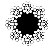
8 x 19 (S)+FC
